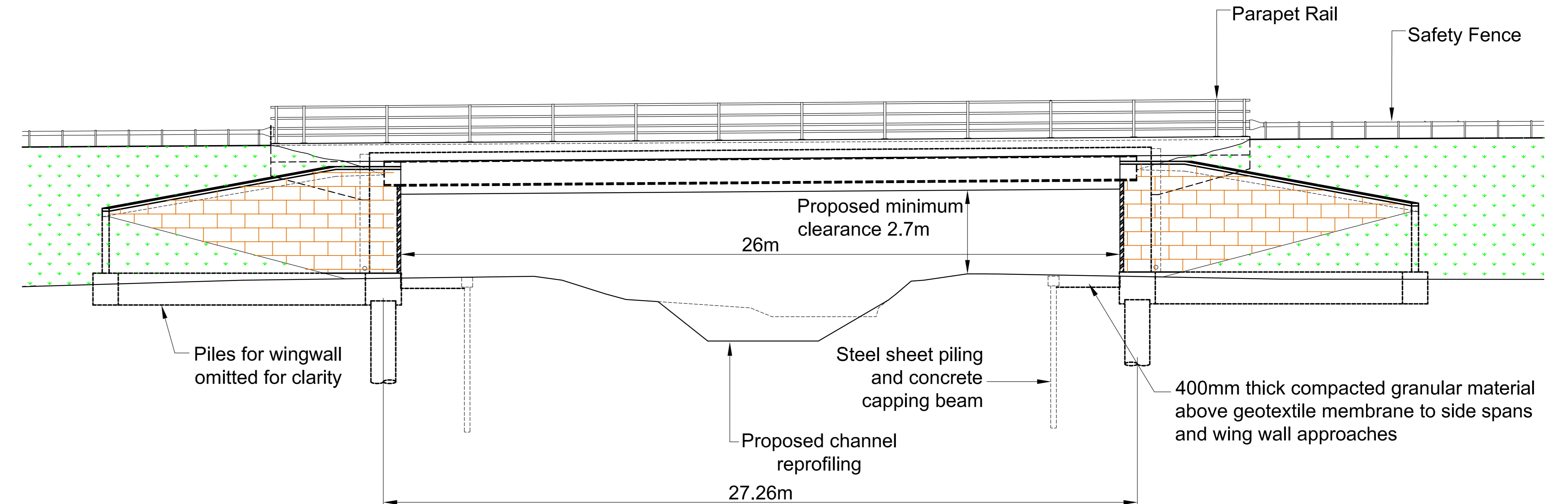
NORTHERN ELEVATION Scale 1:100
