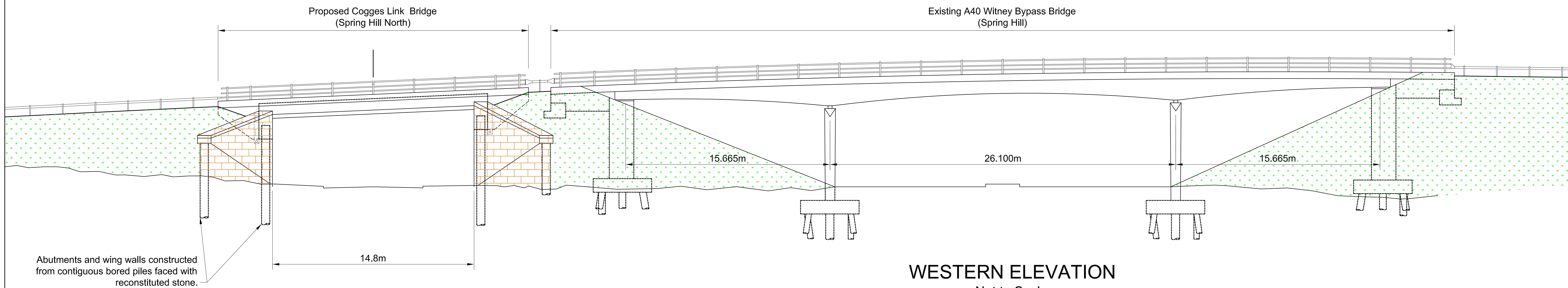
WESTERN ELEVATION Scale 1:100
